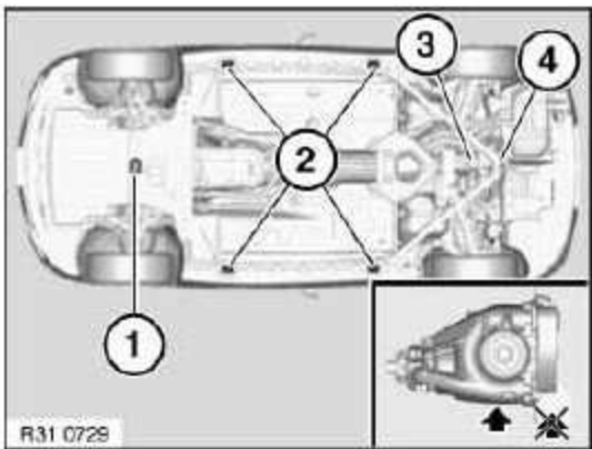
Fig. 12: Identifying Rear Differential, Side Car Jacking Points And Car Jacking Point Courtesy of BMW OF NORTH AMERICA, INC.
